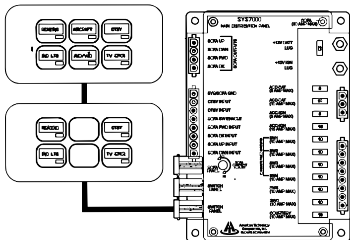
System 7000 Central Fuse Panel
